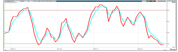
STOCHASTIC
