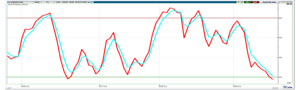
STOCHASTIC
