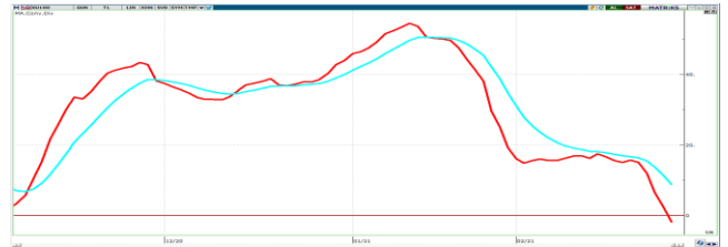
MACD
