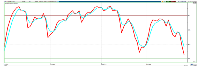
STOCHASTIC
