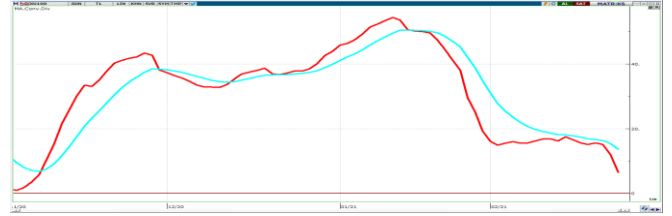
MACD
