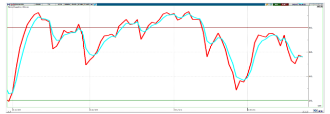
STOCHASTIC
