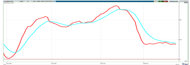
MACD
