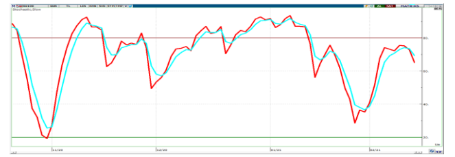
STOCHASTIC
