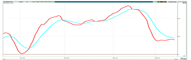
MACD
