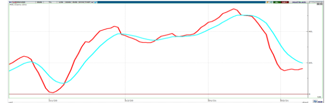
MACD
