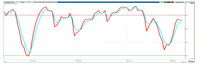
STOCHASTIC
