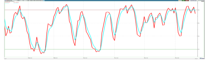
STOCHASTIC
