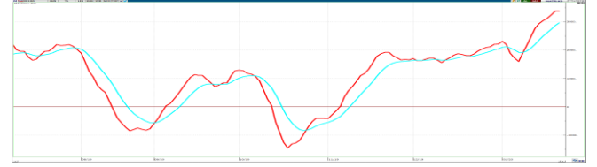
MACD
