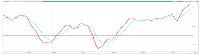
MACD
