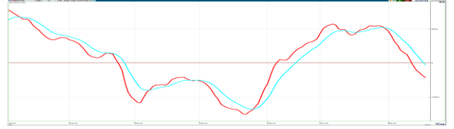
MACD
