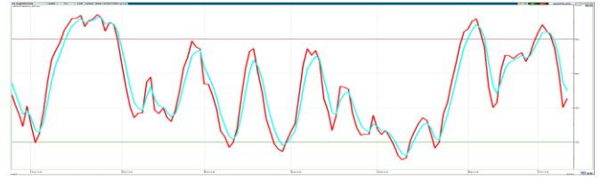
STOCHASTIC
