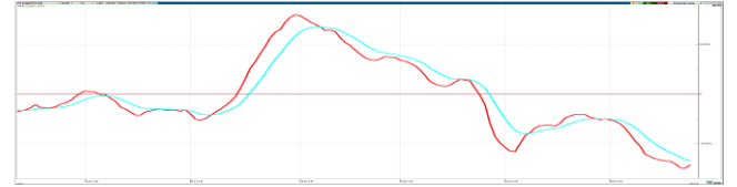
MACD
