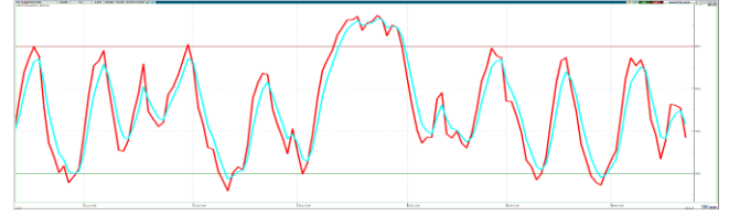
STOCHASTIC
