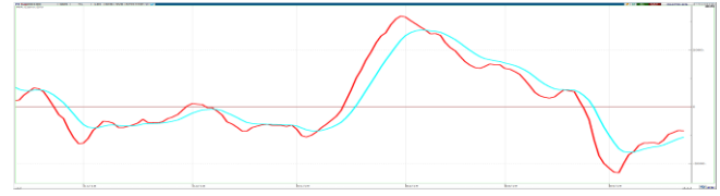
MACD
