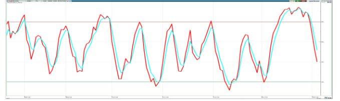
STOCHASTIC
