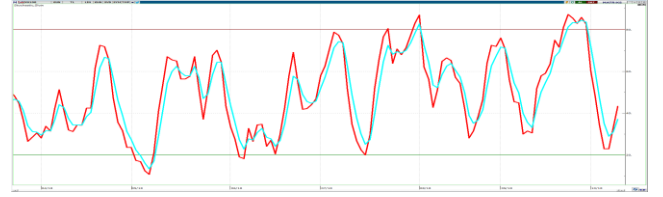
STOCHASTIC
