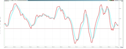
MACD
